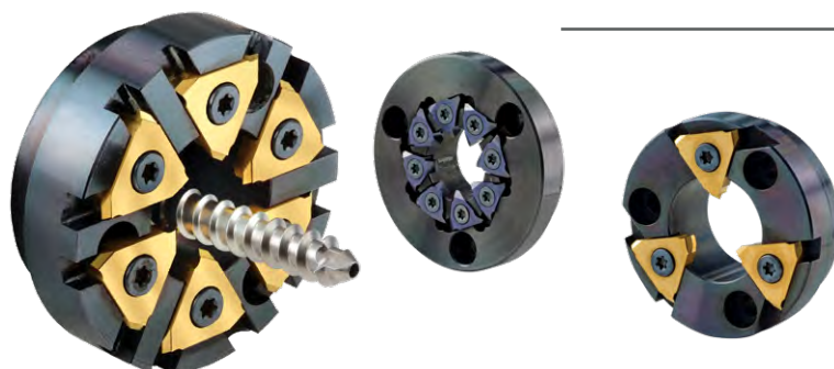
Thread Whirling
